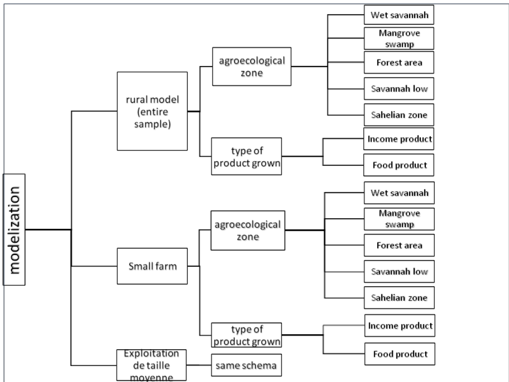
Figure 1: Estimation strategy
